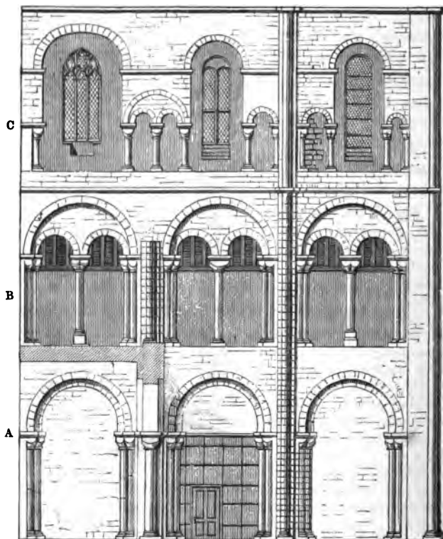
22. Transept, Winchester Cathedral, A.D. 1070—1083.
